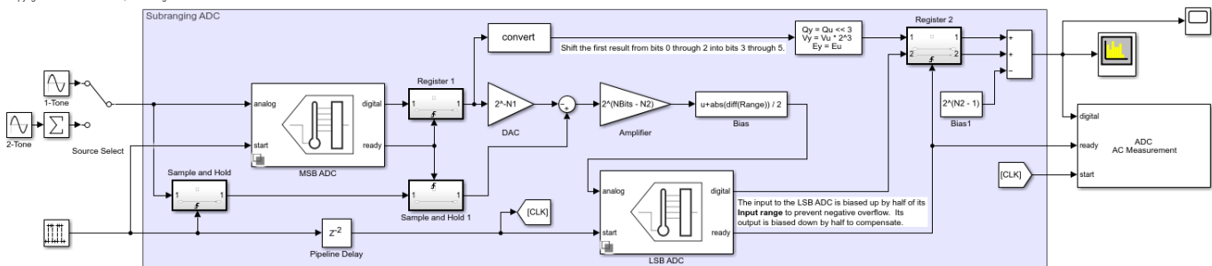
Subranging ADC Example
