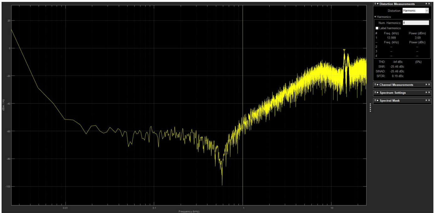
Spectrum analyzer output (50Ksps) from a 2nd order CIFB with noise impairment
